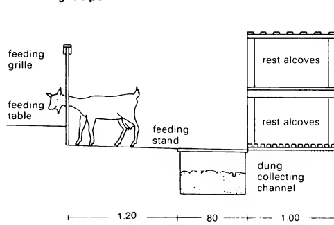
12 Multi-room pen with free-standing rest alcoves
